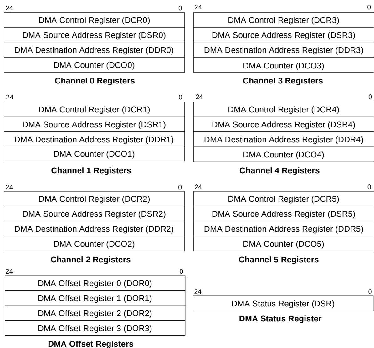
Figure 10-1. DMA Controller Programming Model
