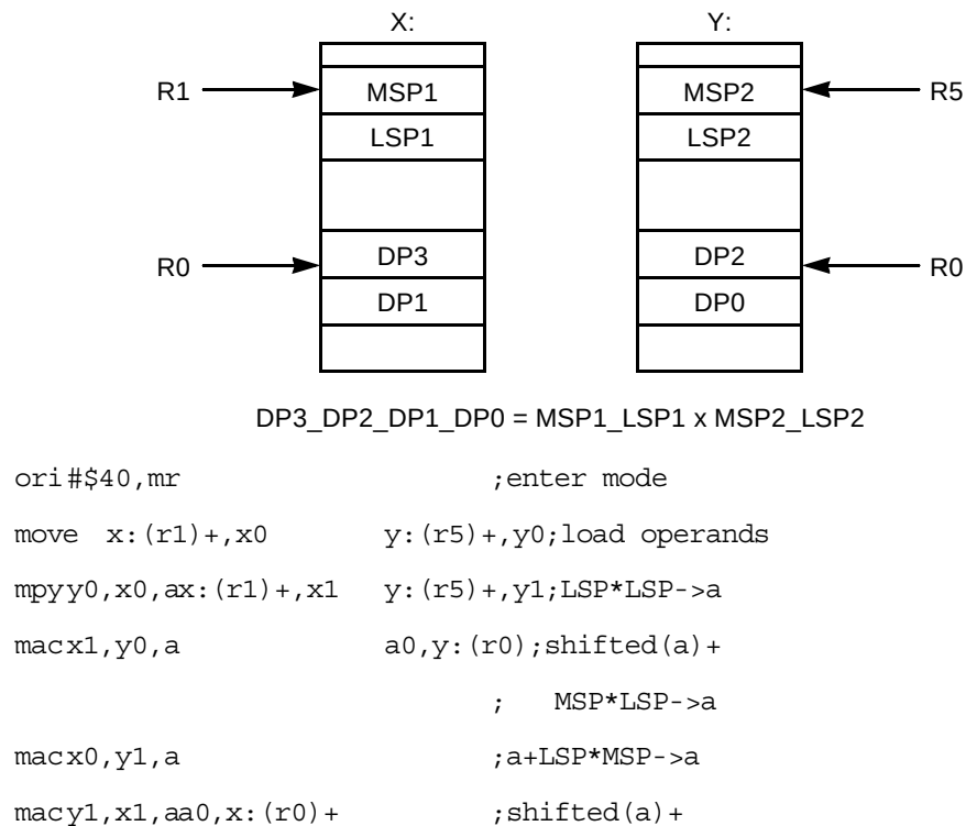
Figure 3-8. Double-Precision Multiply Algorithm
