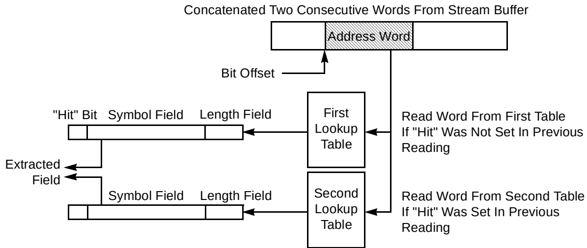
Figure B-5. Parsing Process
